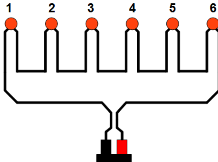
Series Connected Igniters
